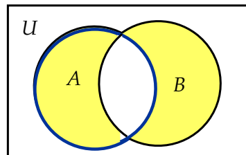
Gambar 1.5: Diagram Venn A \Delta B
