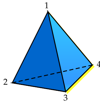
Gambar 2.7: Tetrahedron
