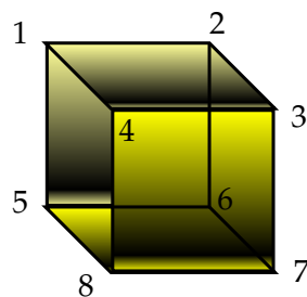
Gambar 2.8: Kubus
