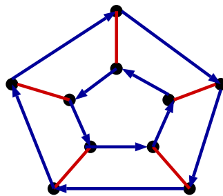
Gambar 3.2: Digraf Cayley
