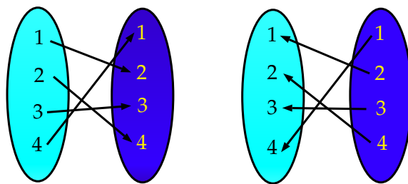
Gambar 1.6: Diagram Fungsi
