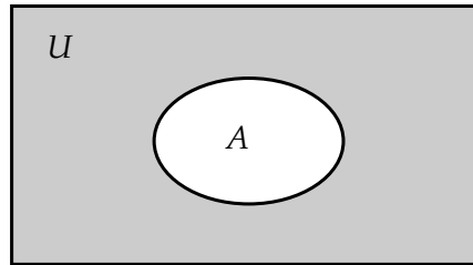
Gambar 1.1: Diagram Venn A^C
